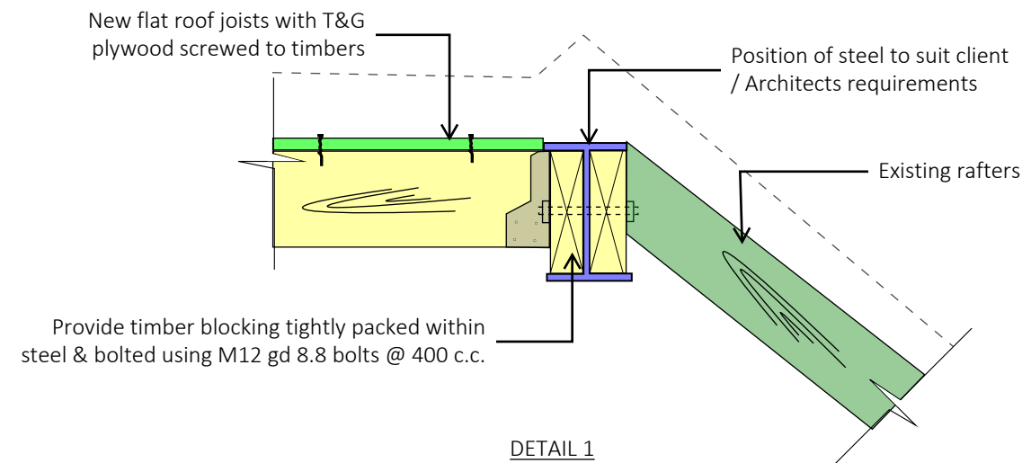
DETAIL 1 UB RIDGE SUPPORT SECTION
