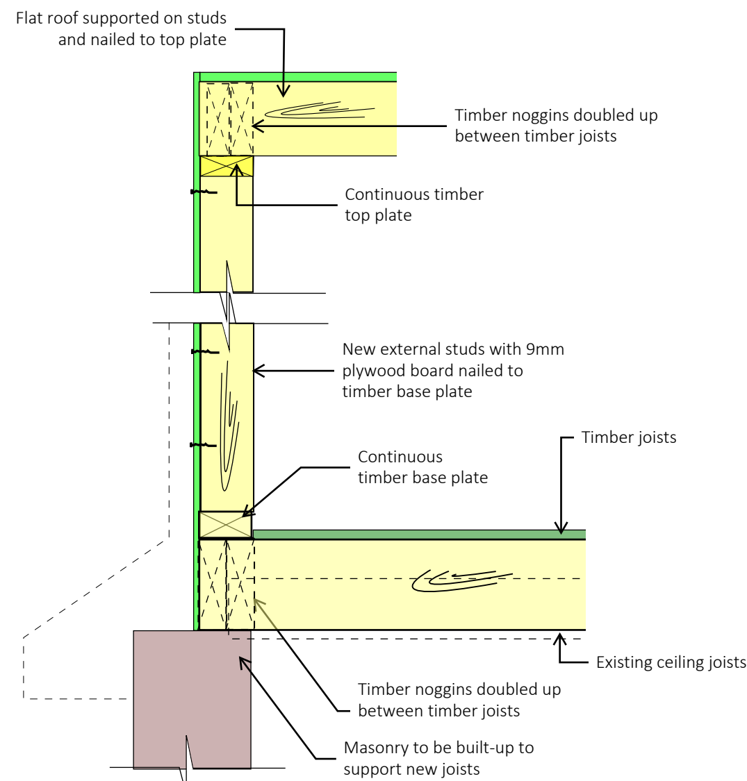
DETAIL 3 REAR STUD WALL TO EXISTING WALL SECTION
