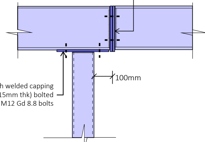
DETAIL 7: BEAM TO COLUMN CONNECTION SECTION
