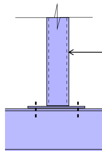
DETAIL 6 COLUMN ON BEAM CONNECTION ELEVATION
