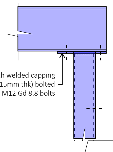
DETAIL 6: SHS / BEAM CONNECTION SECTION
